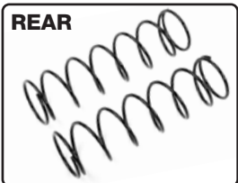
C-00180-291 Shock Spring - Hard - 1.6mm - 84-86mm - 2 pcs
